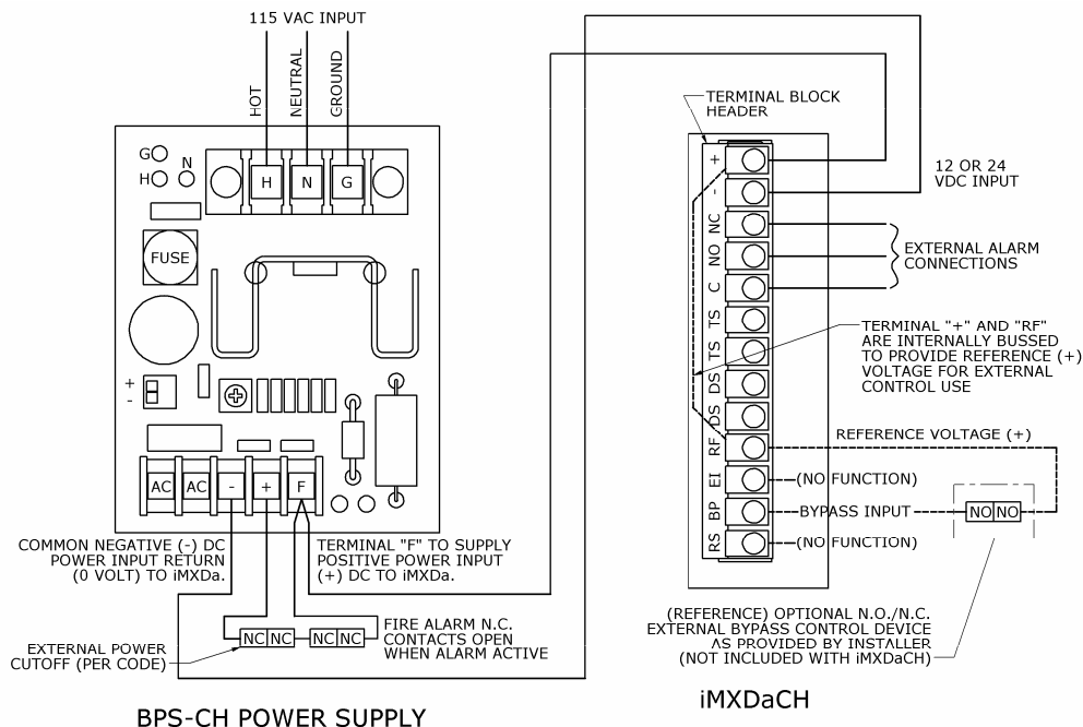
WIRING DIAGRAM FOR iMXDaCH
