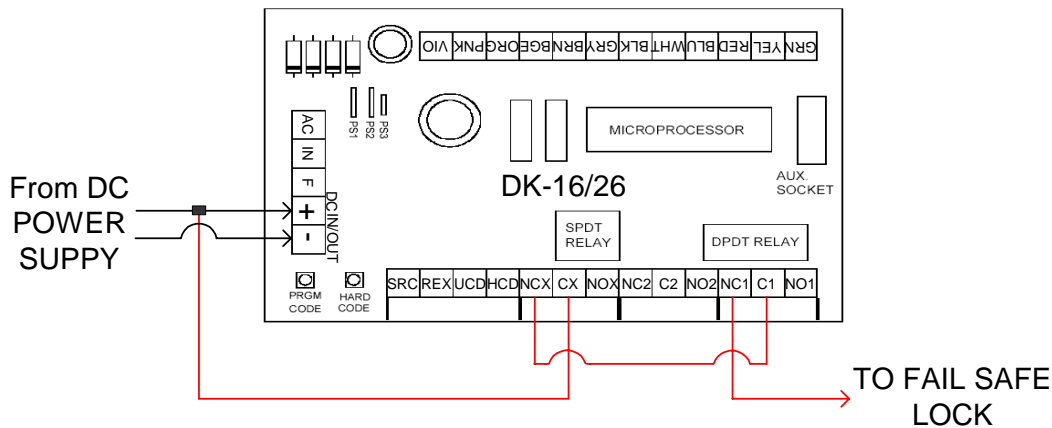
Wiring a DK-16 or DK-26 for HARD CODE Openings & Closings (with a Fail Safe Lock)
