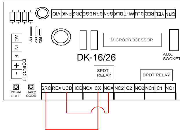
Wiring a DK-16 or DK-26 for HARD CODE Disable of all User Codes
