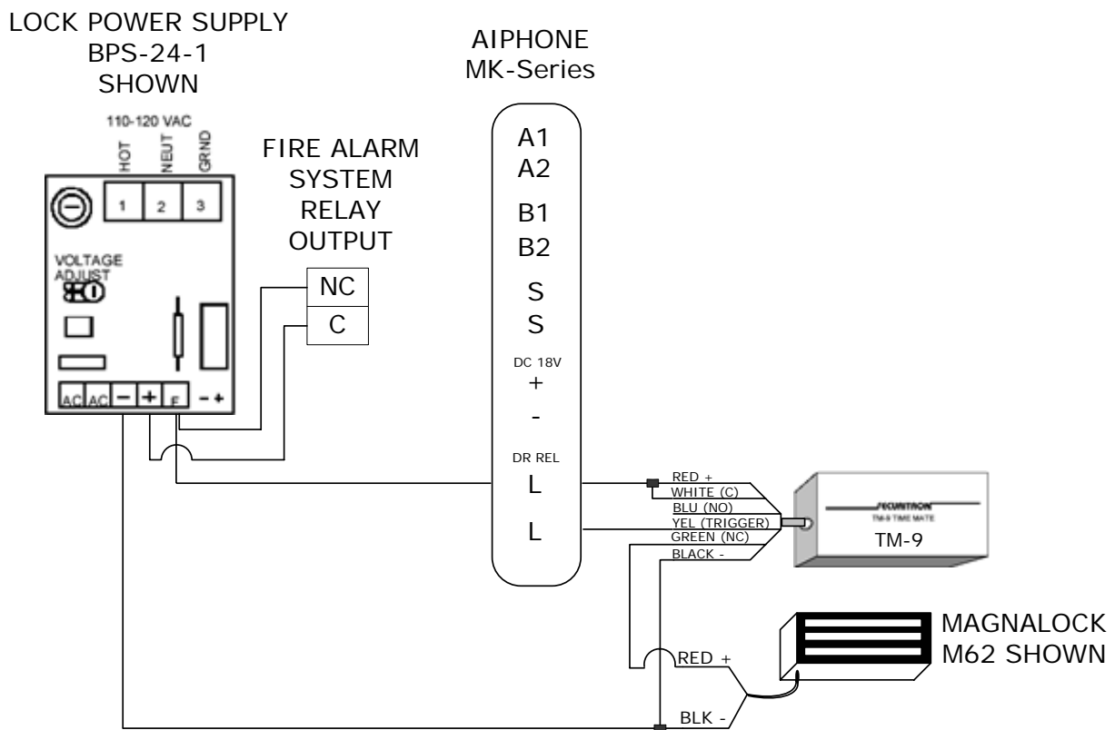
Using the TM-9 for a timed unlock of a Magnalock
